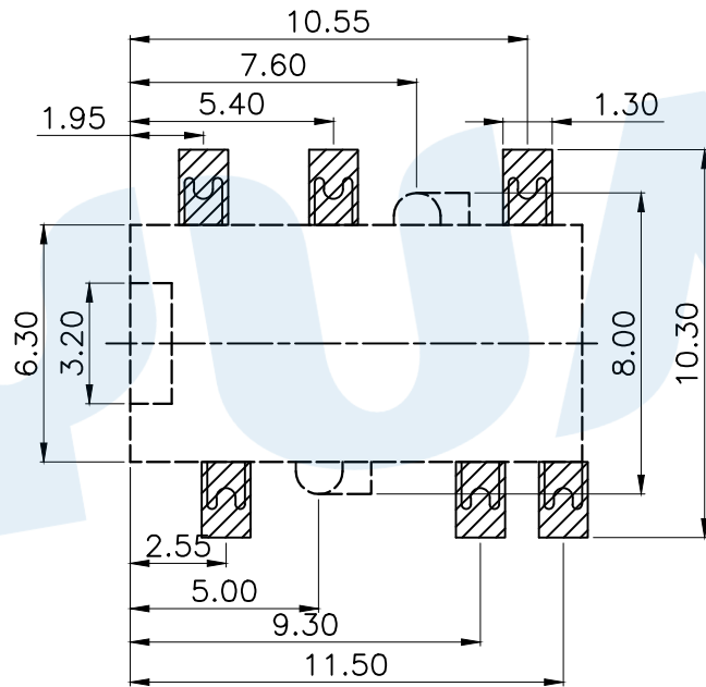
P.C.B LAYOUT(Copper-side view)
