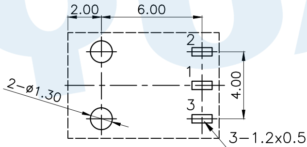
P.C.B LAYOUT(Copper-side view)
