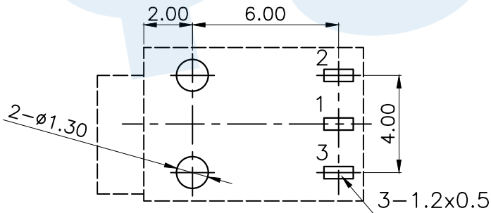
P.C.B LAYOUT(Copper-side view)
